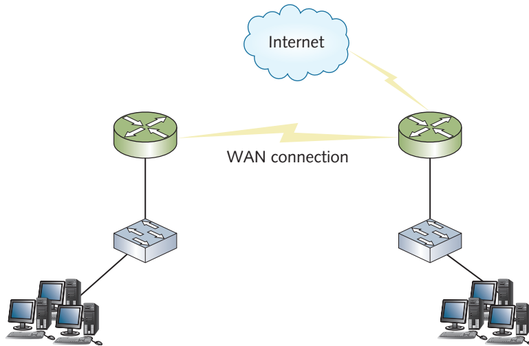
Figure 1-19 A WAN with a connection to the Internet
